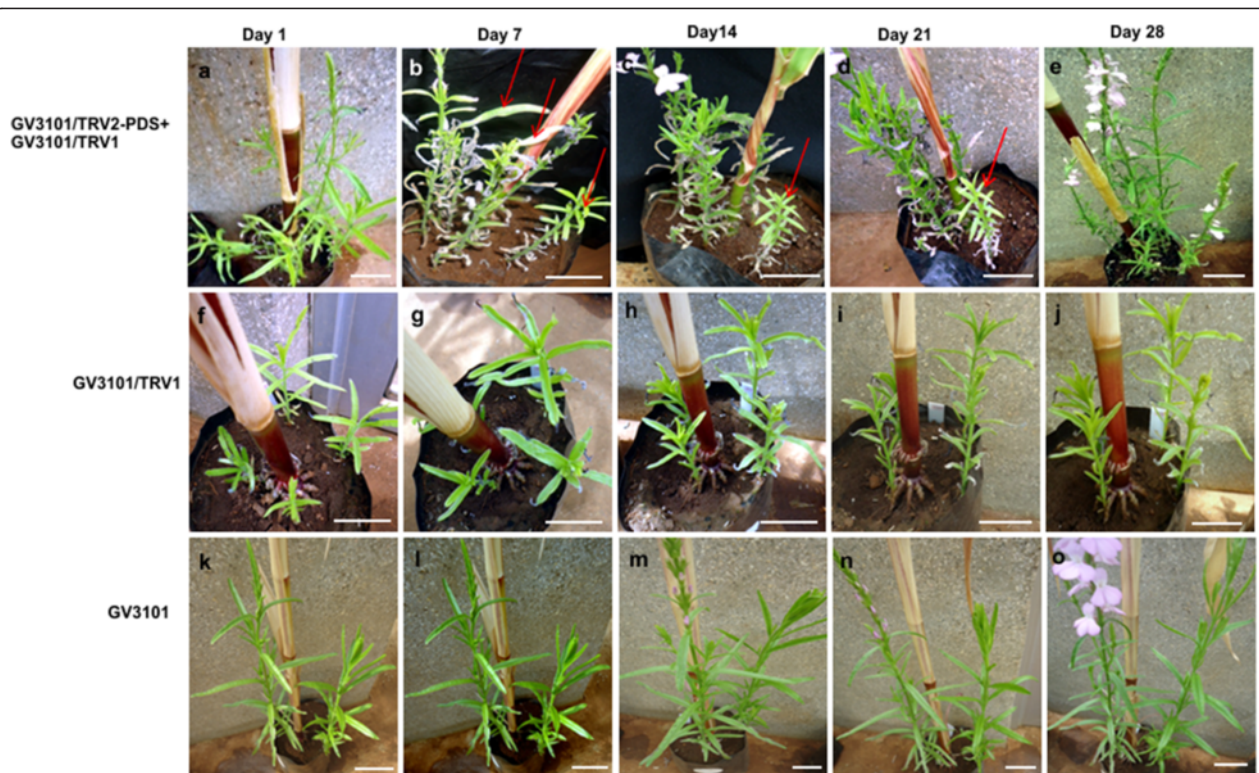
Figure 2 Viral induced gene silencing (VIGS) via agro-infiltration method on S. hermonthica . a, b, c, d, and e are plants agro-infiltrated with Agrobacterium strain GV3101 harbouring TRV2-PDS (GV3101/TRV2-PDS), and mixed in 1:1 ratio with GV3101 containing TRV1 empty vectors (GV3101/TRV1), in days 1, 7, 14, 21 and 28 after agro-infiltration respectively; f, g, h, i and j are plants agro-infiltrated with GV3101 vectors containing TRV1 empty (GV3101/TRV1) in days 1, 7, 14, 21 and 28 after infiltration respectively; k, l, m, n, and o are plants agro-infiltrated with GV3101 only, in days 1, 7, 14, 21 and 28 after agro-infiltration respectively. All scale bars represent 5 cm.
