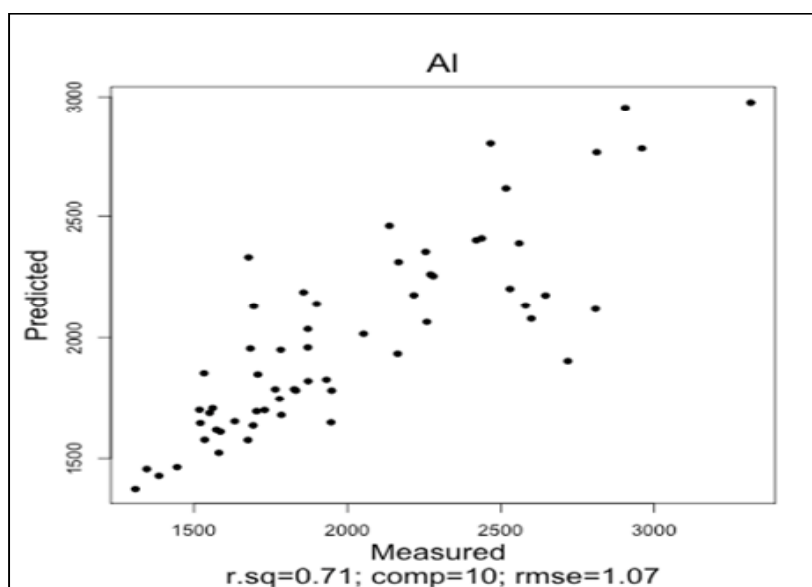
Figure 4.1 : Correlation between measured and predicted values of extractable Al
