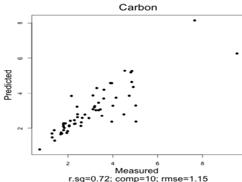
Figure 4.1. Correlation between measured and predicted values of soil organic C
