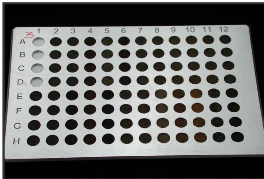
Figure 2 . Sample holder: Aluminum micro plate used at ICRAF Laboratory in Nairobi
