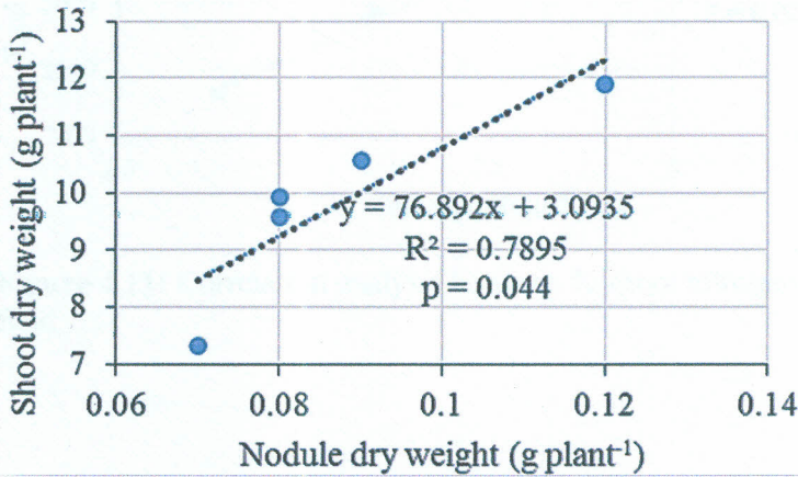
Figure 4.9: Correlation analysis between nodule dry weight and shoot dry weight in the field.
