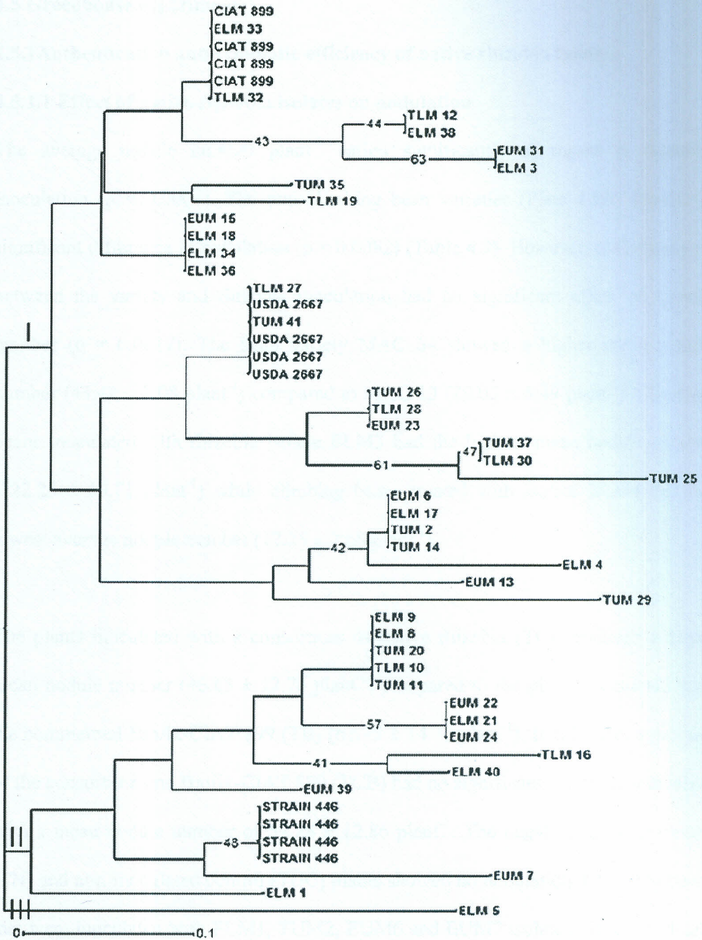
Figure 4.3: Phylogenetic relationship of 41 native rhizobia isolates from Eastern Kenya and 3 reference rhizobia strains (CIAT 899, USDA 2667 and strain 446) inferred using the Neighbor-Joining method. Numbers shown at the nodes of the dendrogram indicate the percentage bootstrap support for 1000 iterations. Only bootstrap values \geq 40\% are shown. Scale bar indicates number of substitutions per site. ELM, Embu Lower Midland; EUM, Embu Upper Midland; TLM, Tharaka Nithi Lower Midland; TUM, Tharaka Nithi Upper Midland.
