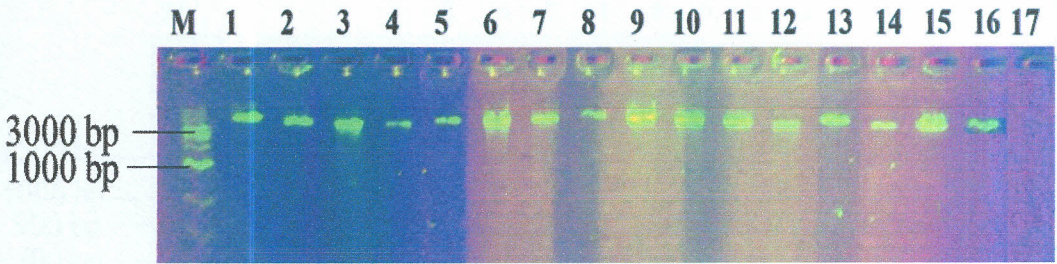
Plate 4.2: Gel electrophoresis of genomic DNA of the selected isolates in 1 % agarose gel. Lane M, 1 kb DNA ladder (Biolabs) used as a molecular marker; Lanes 1 – 13, genomic DNA of native rhizobia isolates (ELM1, TUM2, ELM3, ELM4, ELM5, EUM6, EUM7, ELM8, ELM9, TLM10, TUM11, TLM12, EUM13); Lane 14, CIAT 899; Lane 15, USDA 2667; Lane 16, strain 446; Lane 17, Negative control.
