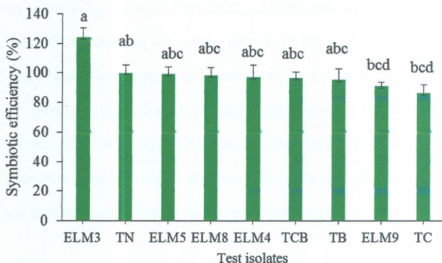
Figure 4.4: Symbiotic efficiencies of native rhizobia isolates from Eastern Kenya. ELM3, ELM4, ELM5, ELM8 and ELM9, Native rhizobia isolates which nodulated; TC, Consortium of native rhizobia; TB, Commercial inoculant (Biofix-CIAT 899); TN, Negative control with nitrogen treatment; TCB, Biofix-CIAT 899 combined with consortium.
