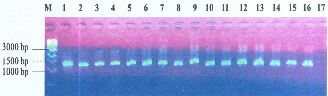
Plate 4.3: PCR amplified 16S rDNA of the isolates in 1 % agarose gel. Lane M, 1 kb DNA ladder (Biolabs); Lanes 1 – 13, genomic DNA of selected native rhizobia isolates (ELM1, TUM2, ELM3, ELM4, ELM5, EUM6, EUM7, ELM8, ELM9, TLM10, TUM11, TLM12, EUM13); Lane 14, CIAT 899; Lane 15, USDA 2667; Lane 16, strain 446; Lane 17, Negative control.
