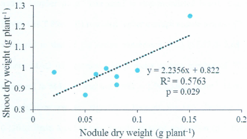
Figure 4.5: Correlation analysis between shoot dry weight and nodule dry weight.
