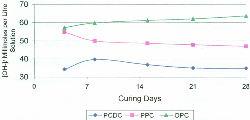
Figure 4.2: OH - Concentration Change as a Function of Curing Period
