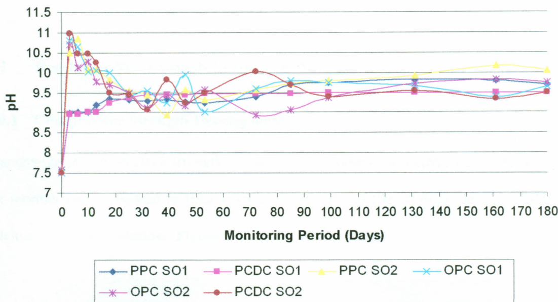
Figure 4.36: pH Measurements in Simulated Sulphate Solutions
