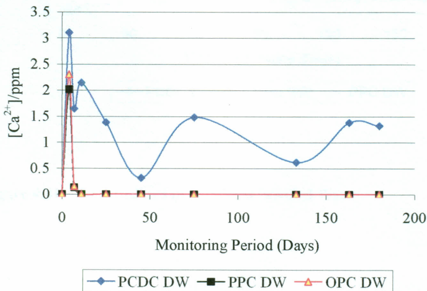
Figure 4.39: \text{Ca}^{2+} Analyses in Simulated Distilled Water
