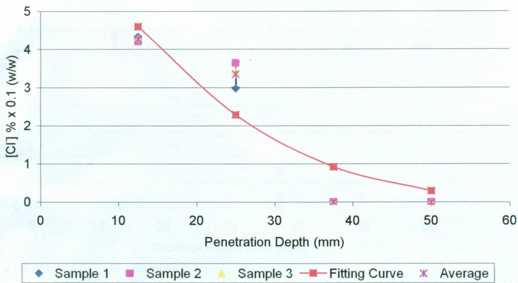
Figure 7.3: Error Function fitting for OPC-25 % PFA(w/c ratio 0.73), D_{app}= 2.01 \times 10^{-11} \text{ m}^2/\text{s} , and C_s = 0.76 \text{ \%} ( r^2 = 0.87 )
