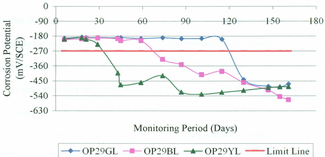
Figure 4.21: Corrosion Potential Verses Time for OPC at w/c of 0.85
