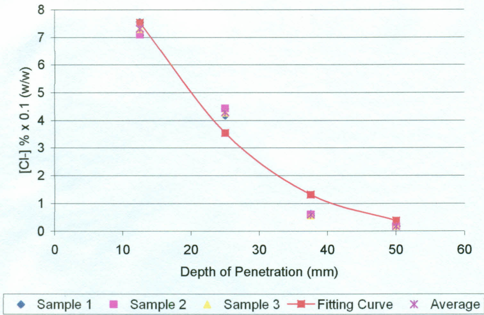
Figure 7.7: Error Function fitting for PCDC (w/c ratio 0.8), D_{app} = 1.81 \times 10^{-11} \text{ m}^2/\text{s} , and C_s = 1.285 \% ( r^2 = 0.968 )
