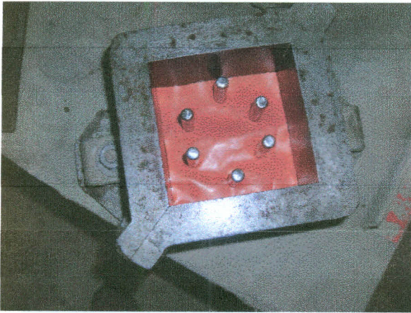
Plate 3.2: PVC block with Polythene sheet lining in the Mortar Cube
