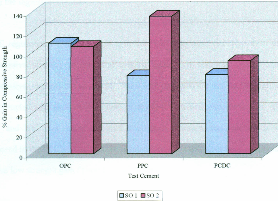
Figure 4.31: Percent Gain in Compressive Strength versus Test Cement
