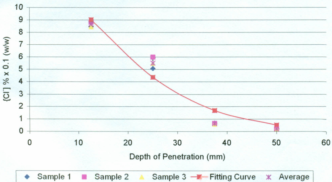
Figure 7.8: Error Function fitting for PCDC (w/c ratio 0.85), D_{app} = 1.91 \times 10^{-11} \text{ m}^2/\text{s} , and C_s = 1.513 \% ( r^2 = 0.9506 )
