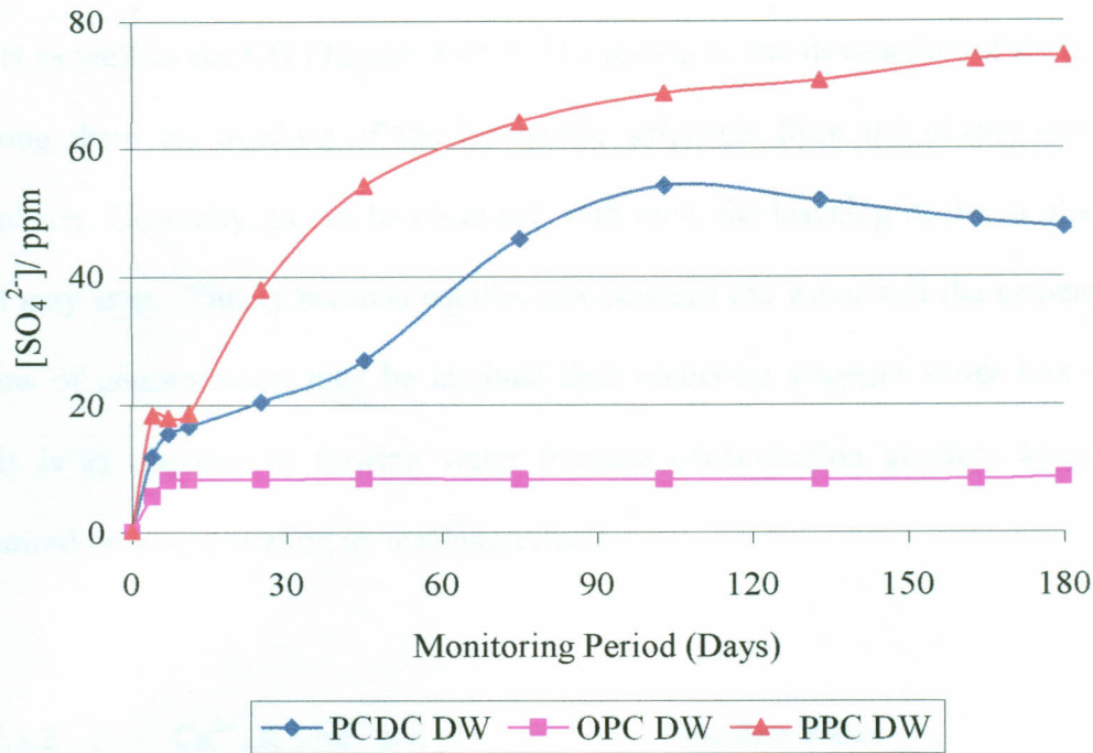
Figure 4.38: \text{SO}_4^{2-} Analyses in Distilled Water
