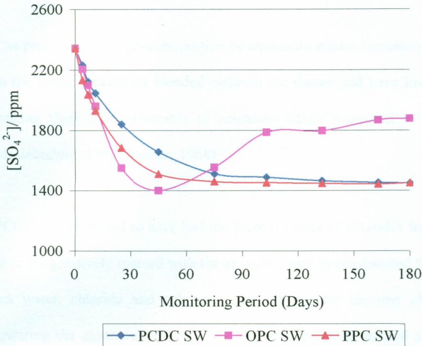
Figure 4.45: \text{SO}_4^{2-} Analyses in Sea Water
