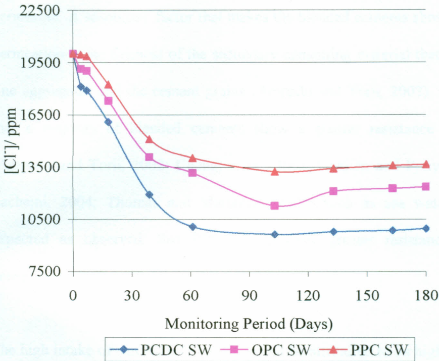
Figure 4.44: \text{Cl}^- Analyses in Sea Water
