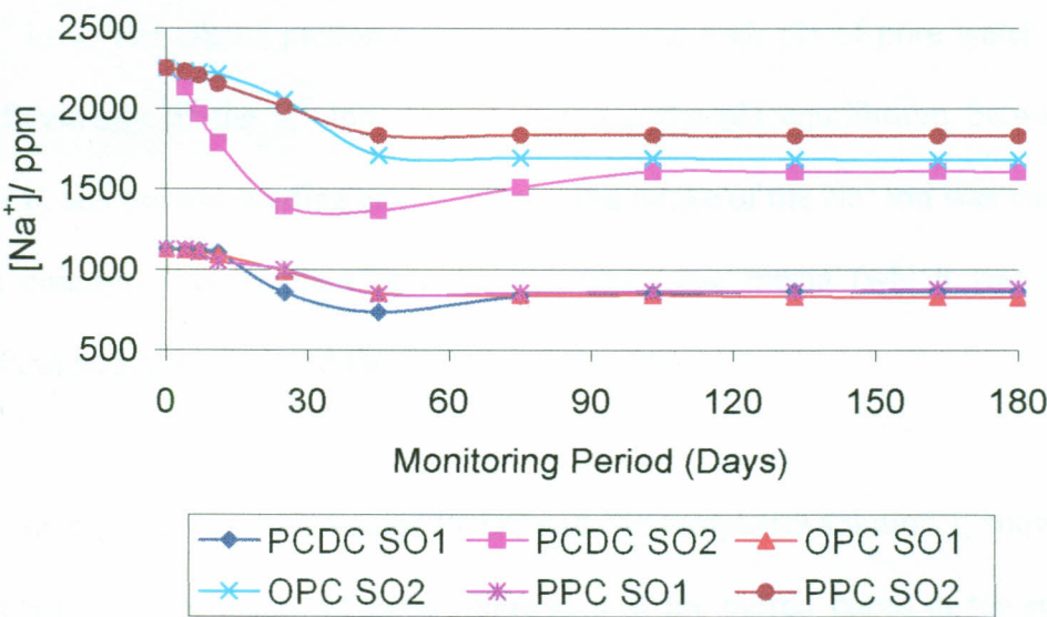
Figure 4.35: Na^+ Analyses from Simulated Sulphate Solutions
