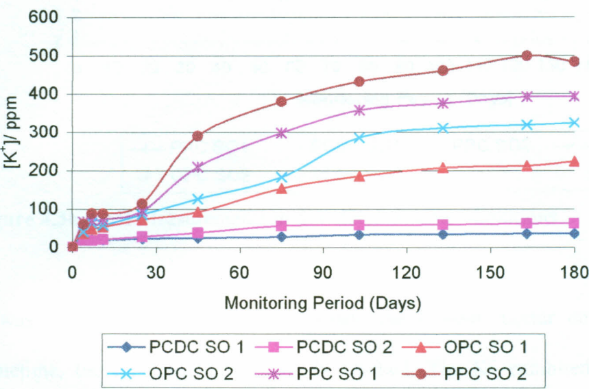
Figure 4.34: K^+ Analyses in Sulphate Simulated Solution
