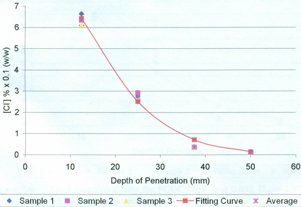
Figure 7.6: Error Function fitting for PCDC (w/c ratio 0.73), D_{app} = 1.34 \times 10^{-11} \text{ m}^2/\text{s} , and C_s = 1.219 \% ( r^2 = 0.9934 )
