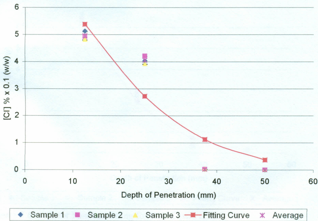
Figure 7.4: Error Function fitting for OPC-25 % PFA(w/c ratio 0.80), D_{app}= 2.09 \times 10^{-11} \text{ m}^2/\text{s} , and C_s = 0.879 \text{ \%} ( r^2 = 0.8505 )
