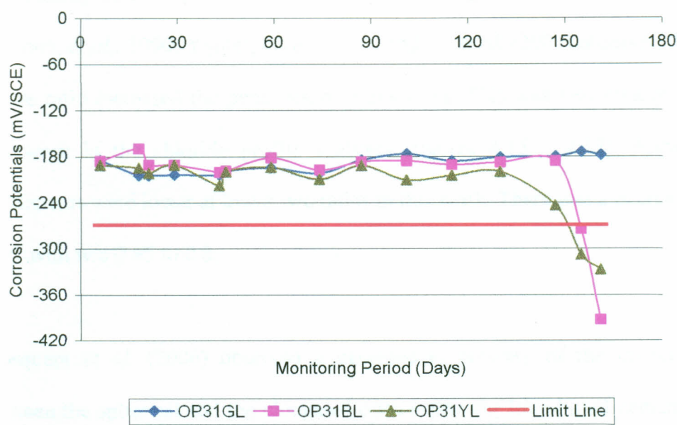
Figure 4.25: Corrosion Potential Verses Time for OPC at w/c of 0.80
