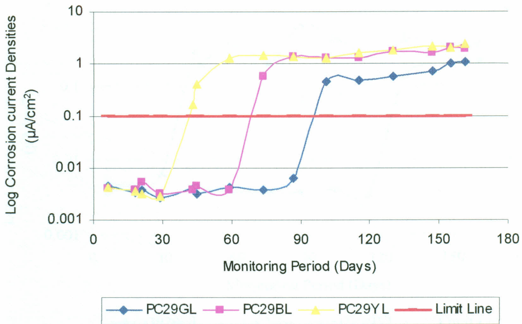
Figure 4.20: Log Corrosion Current Densities Verses Time for PCDC at w/c 0.85
