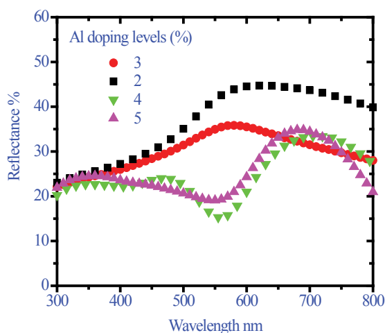
Figure 3: Spectral graph of reflectance % in the visible, IR, and UV regions against wavelength (nm) for different doping levels of AZO.
