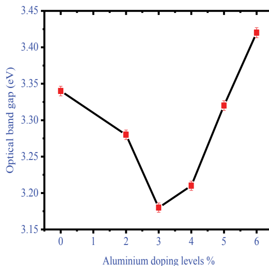
Figure 5: Variation of optical band gap for ZnO:Al with various doping levels of Aluminum (%).
