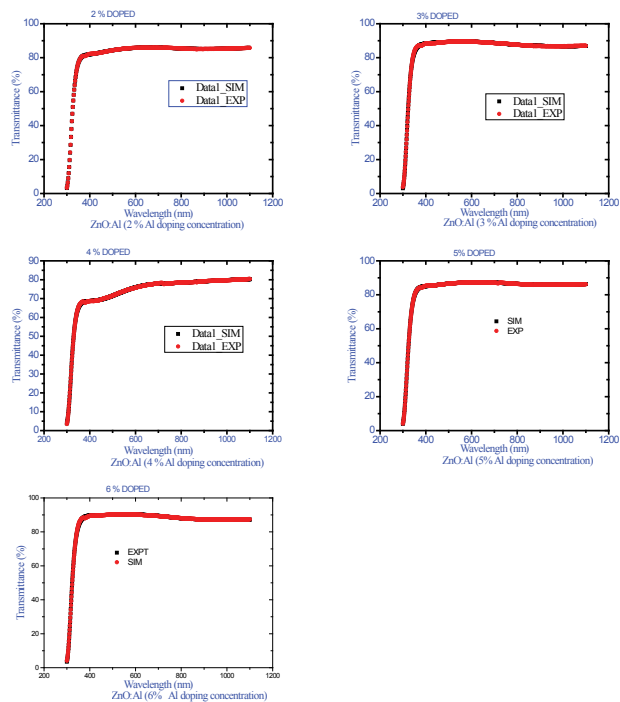
Figure 4: Doping Concentration of Al: ZNO and transmittance spectra for ZnO doped with Al at various Al doping levels.
