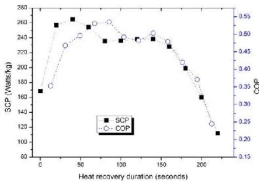
Fig. 5 Variation of cycle COP and SCP with heat recovery duration
