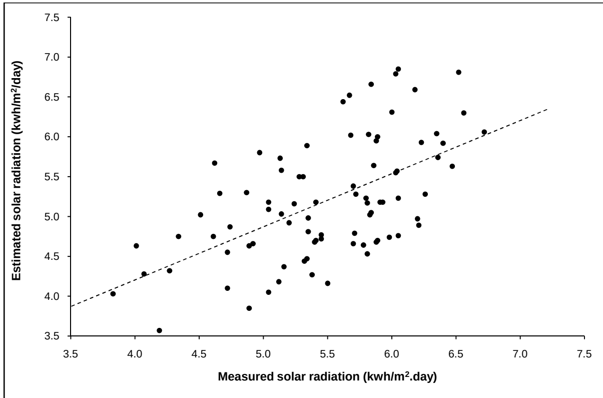
Figure 5: Scatter plot of measured versus estimated solar radiation for the validation set (n=84)
