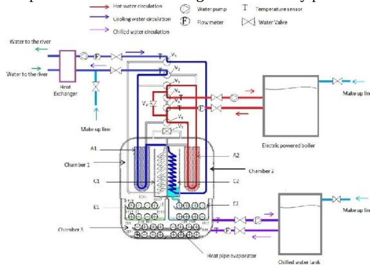
Fig.1 A schematic diagram of experimental set up(Ishugah, Wang et al. 2014)
