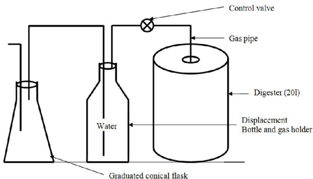
Figure 1: Schematic representation of experimental set up
