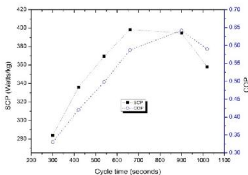
Fig. 2 Variation of SCP and COP with adsorption/desorption duration
