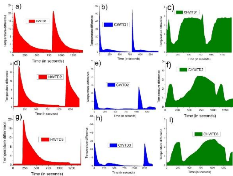
Fig. 4 Temperature difference between inlet and outlet of cooling water
