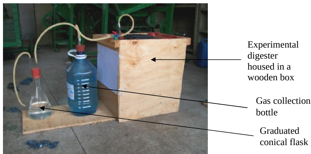
Figure 3: Experimental set up showing gas collection system
