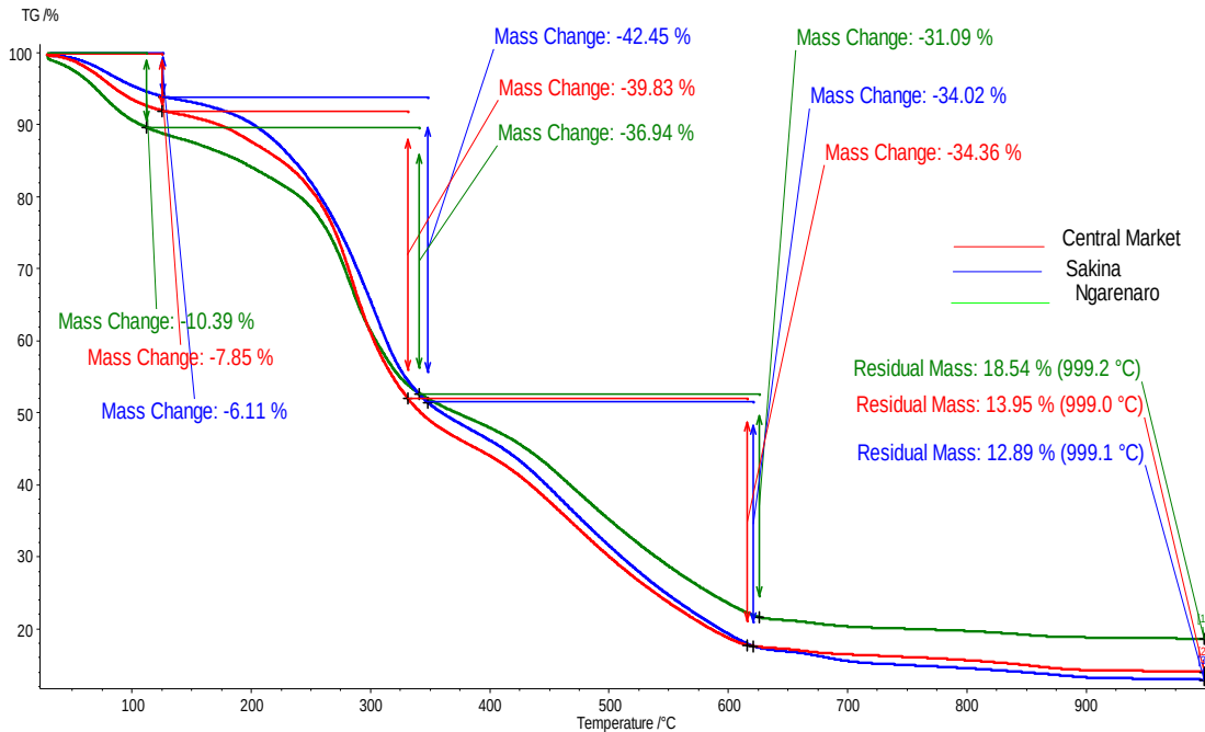
Figure 4: TGA graphs of Municipal solid waste from three locations in Arusha city
