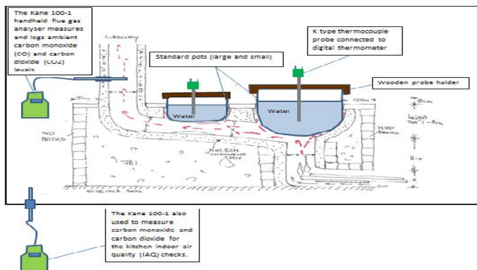
Figure 8: Testing Rig of the proposed mud-brick cook-stove
