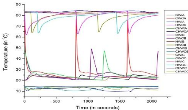
Fig. 3 Temperature profile at different heat recovery times
