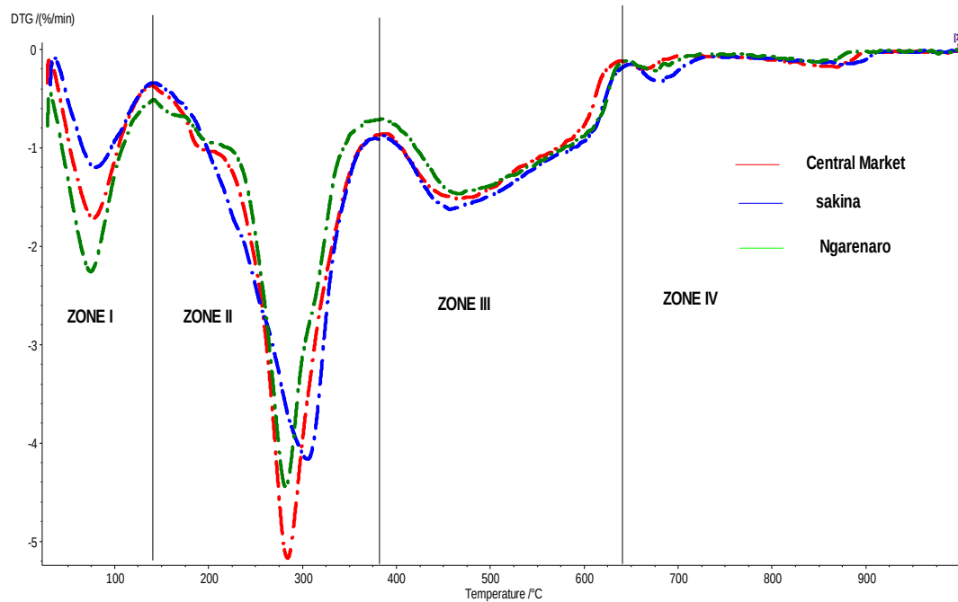
Figure 5: DTG of municipal solid waste from three locations in Arusha City
