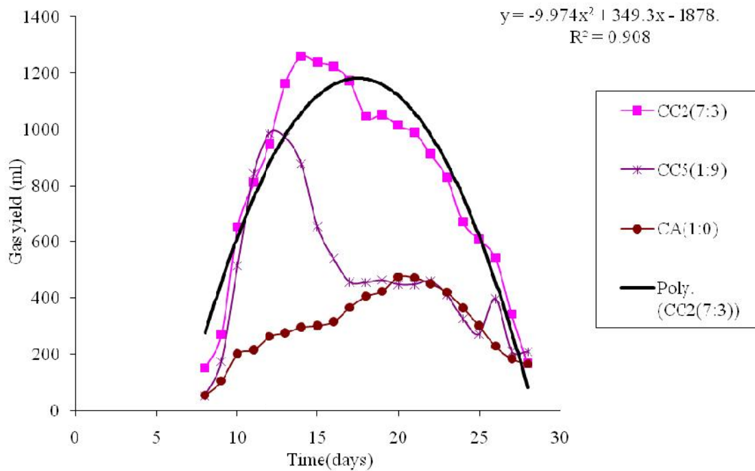
Figure 4: Daily variation of gas produced for mixture ratios CC and CA
