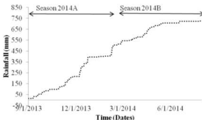
Figure 2. Cumulative daily rainfall during the study period (seasons A2014 and B2014). Source: RAB Karama Research Station.
