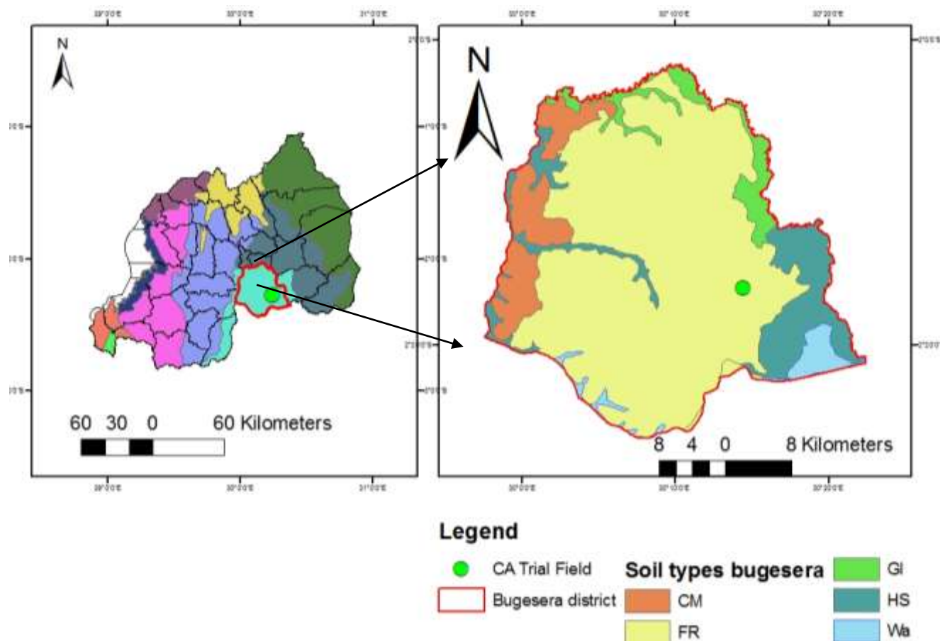
Figure 1. Map of Bugesera District showing research sites and their dominant soils (CM= Cambisols, FR=Ferralsols, GL=Gleysols, HS=Histosols, Wa=Water).
