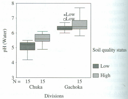
Figure 2d. Comparisons of soil reaction (pH).
