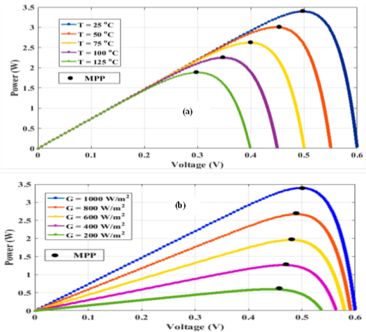
Figure 1. P-V curve for temperature and irradiance variation [adapted from [7]]
