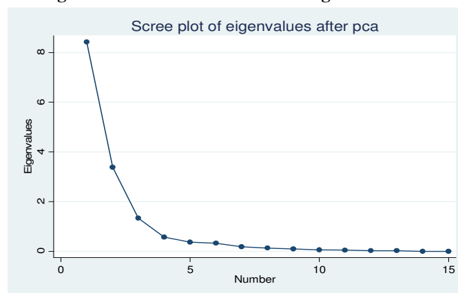
Figure 3: Scree plot
