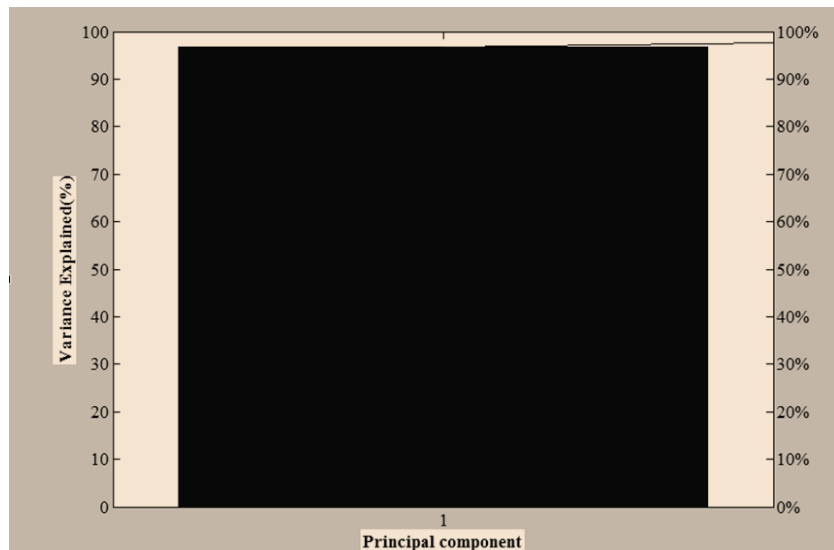
Fig. 1. Scree plot
