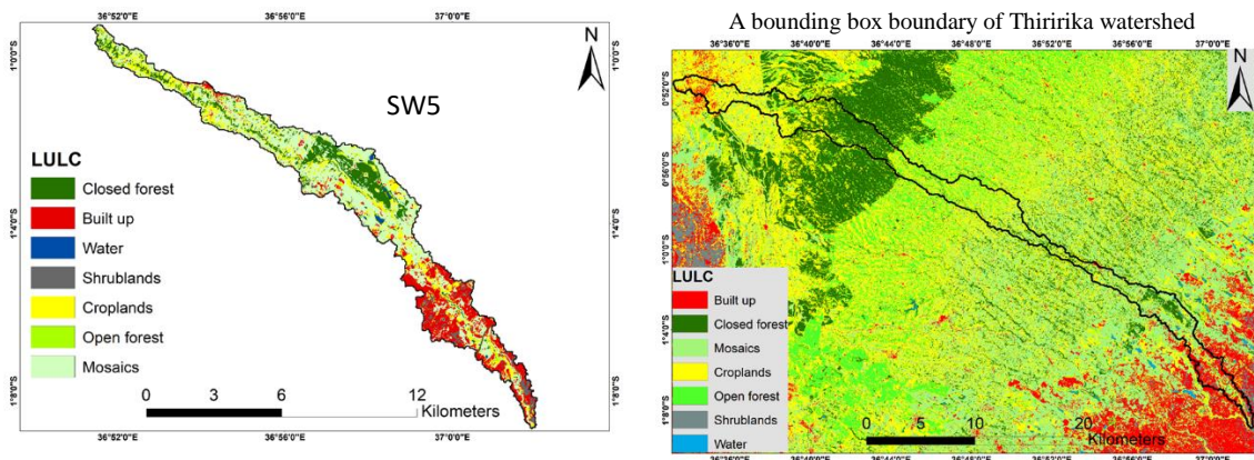
Figure 3: Thiririka sub-watersheds land use and land cover classification maps
