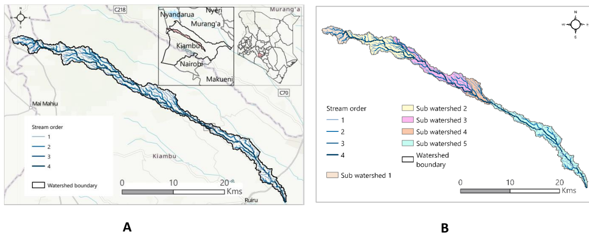
Figure 1: (A) Thiririka watershed and stream network (B) Delineated sub watersheds
