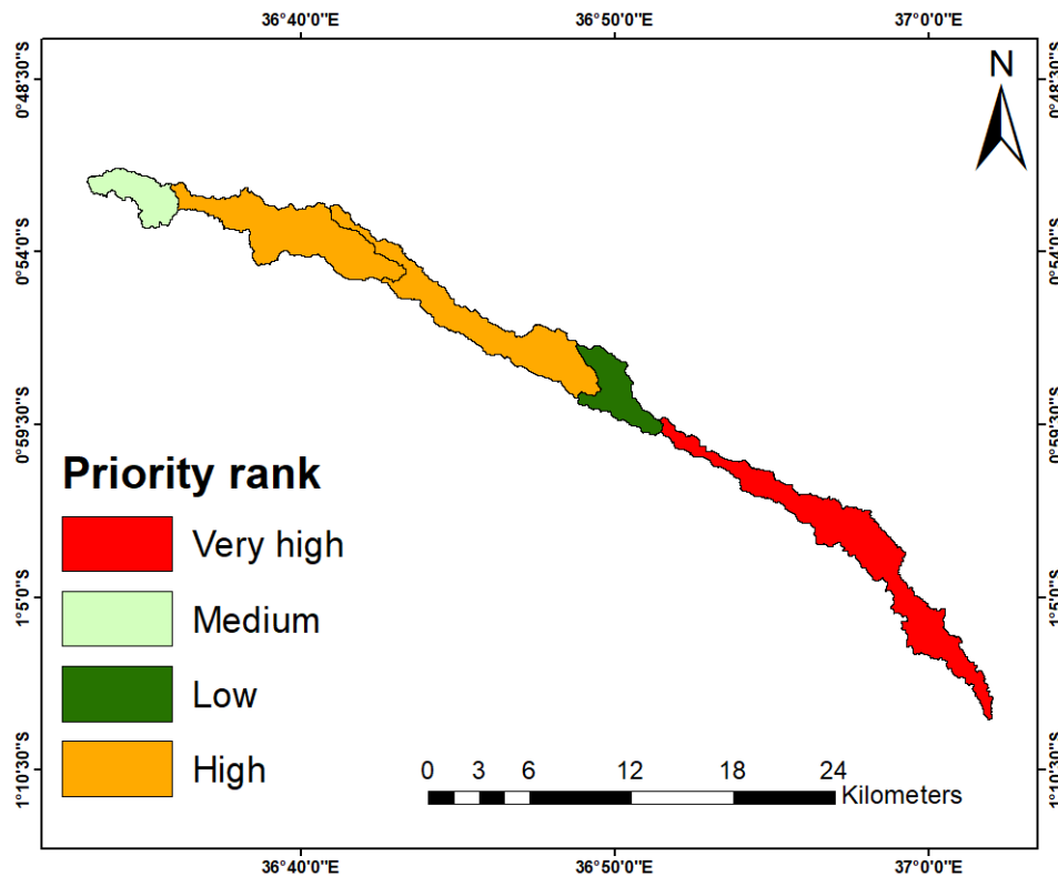
Figure 4: Thiririka sub-watersheds soil erosion susceptibility map, the ranks were derived from mean compound value of basin morphometric parameters and land use / land cover.
