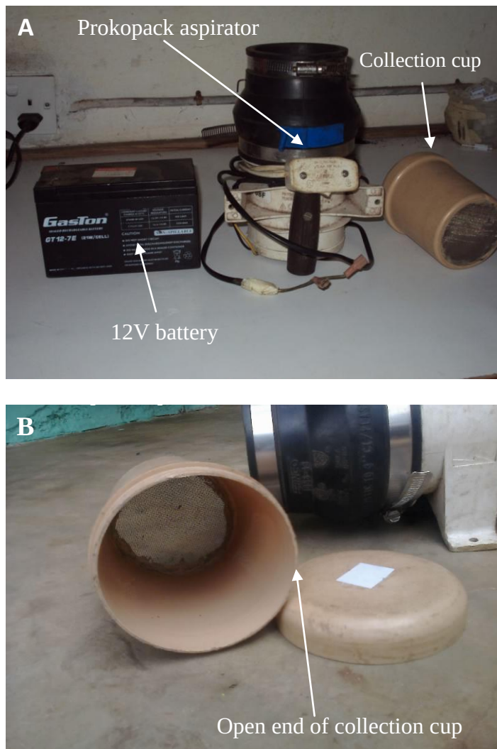
Figure 3: (A) Picture of the prokopack aspirator, 12V battery and plastic collection cup; (B) shows a picture of the open end of the collection cup
