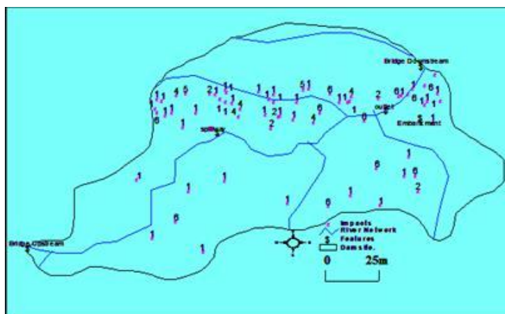
Figure 3. Spatial distribution of hydro-geomorphologic impacts in Muooni Dam (Luwesi, 2010)
