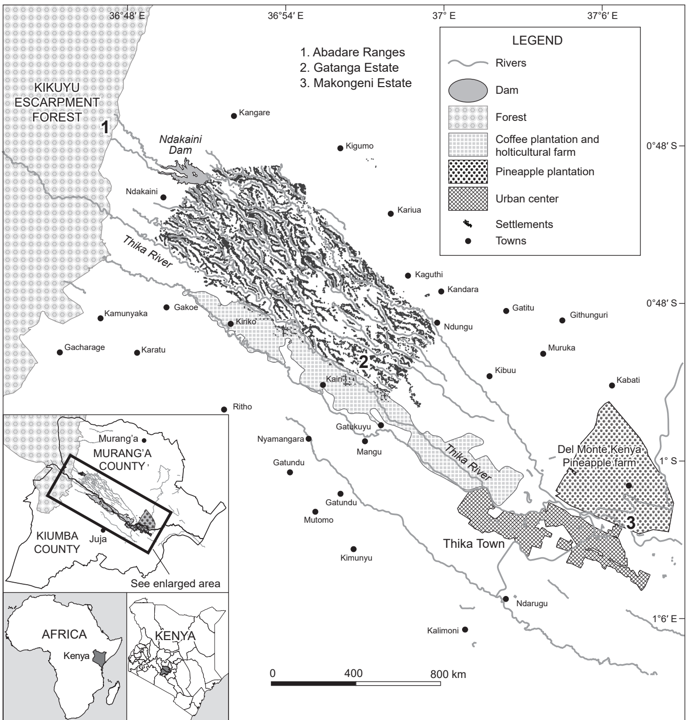
Figure 1: Map of study area showing sampling sites 1, 2 and 3 within the Thika catchment in Murang'a county, Kenya. Site 1 was surrounded by natural forest in the Aberdare ranges, Site 2 by agricultural farmlands and Site 3 by industrial and urban settlements
