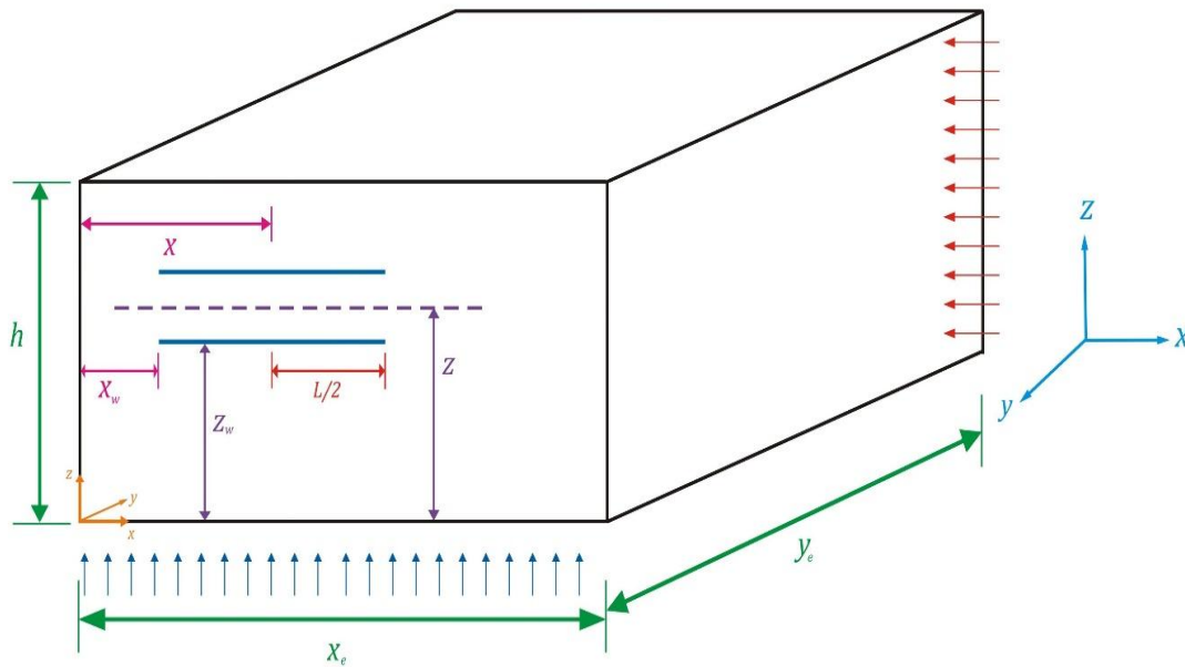
Figure 1: Horizontal well acting in an infinite reservoir
