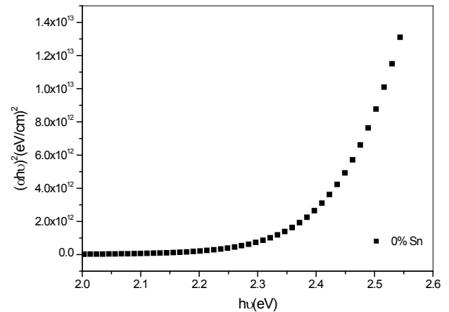
Figure 4. Plot of (\alpha h\nu)^2 versus photon energy h\nu for undoped CdO thin films
