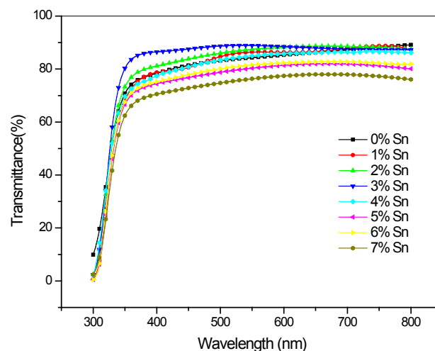
Figure 1. Transmittance spectra of 0-7% Sn doped CdO
